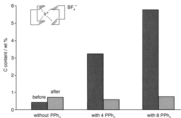
Figure 4. Carbon content of dehydrogenation catalysts before (black) and after the reaction (shaded).
