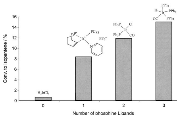
Figure 1. Correlation between the number of phosphine ligands and the activity of the catalyst for the dehydrogenation of isopentane at 400°C.
