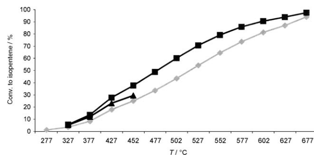
Figure 5. Calculation of the thermodynamic equilibrium of the dehydrogenation reaction of isopentane at different temperatures (light gray: Aspen, dark gray: HSC Chemistry, black: experimental results).
