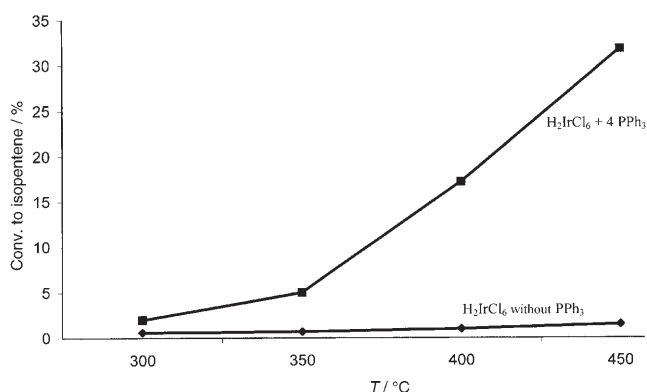
Figure 2. Comparison of the activity of \text{H}_2\text{IrCl}_6 on silica gel without \text{PPh}_3 and with 4 equiv \text{PPh}_3 depending on the reaction temperature.
