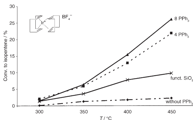
Figure 3. Comparison of conversion rates of catalysts with and without triphenylphosphine.
